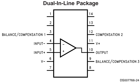
Top View Order Number LM118J/883 (Note 13) See NS Package Number J14A
