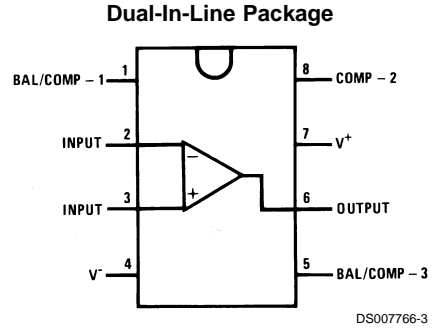
Top View Order Number LM118J-8/883 (Note 13), LM318M or LM318N See NS Package Number J08A, M08A or N08B
