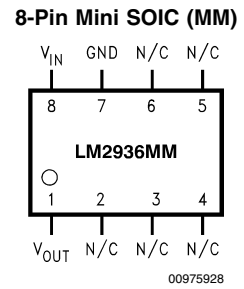
Top View Order Number LM2936MM-5.0 See NS Package Number MUA08A
