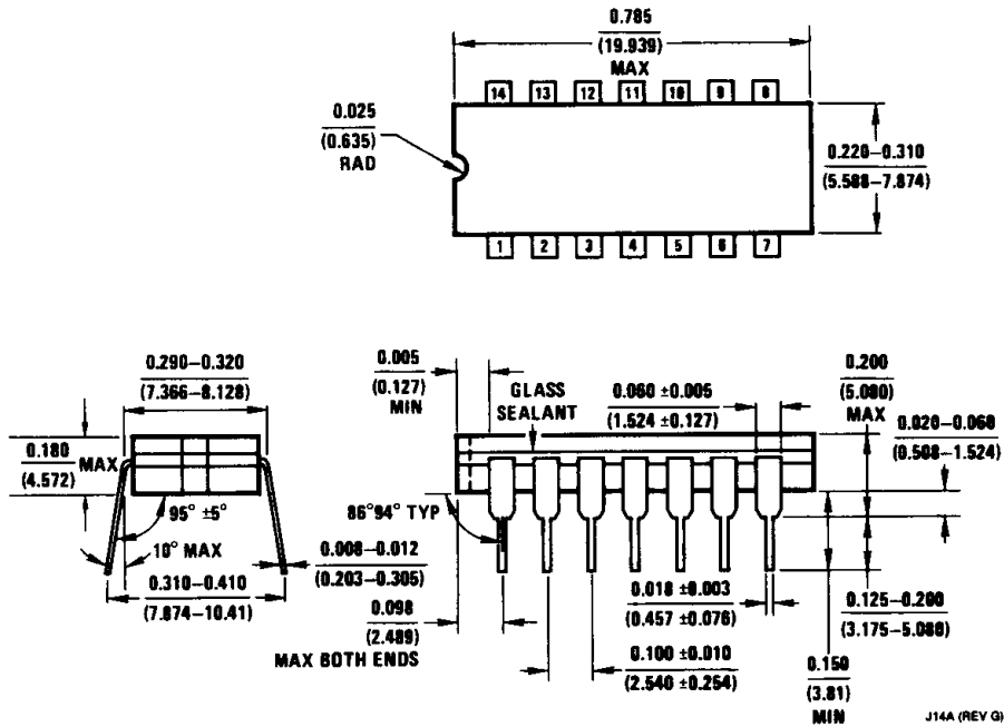
Order Number ADC08234BIJ, ADC08234CIJ or ADC8234CMJ NS Package Number J14A
