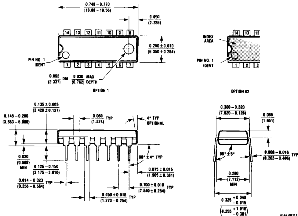
Order Number ADC08234BIN or ADC08234CIN NS Package Number N14A
