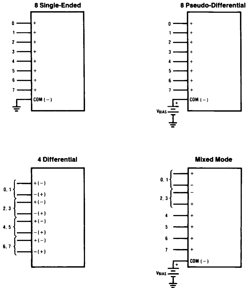
FIGURE 1. Analog Input Multiplexer Options for the ADC08238
