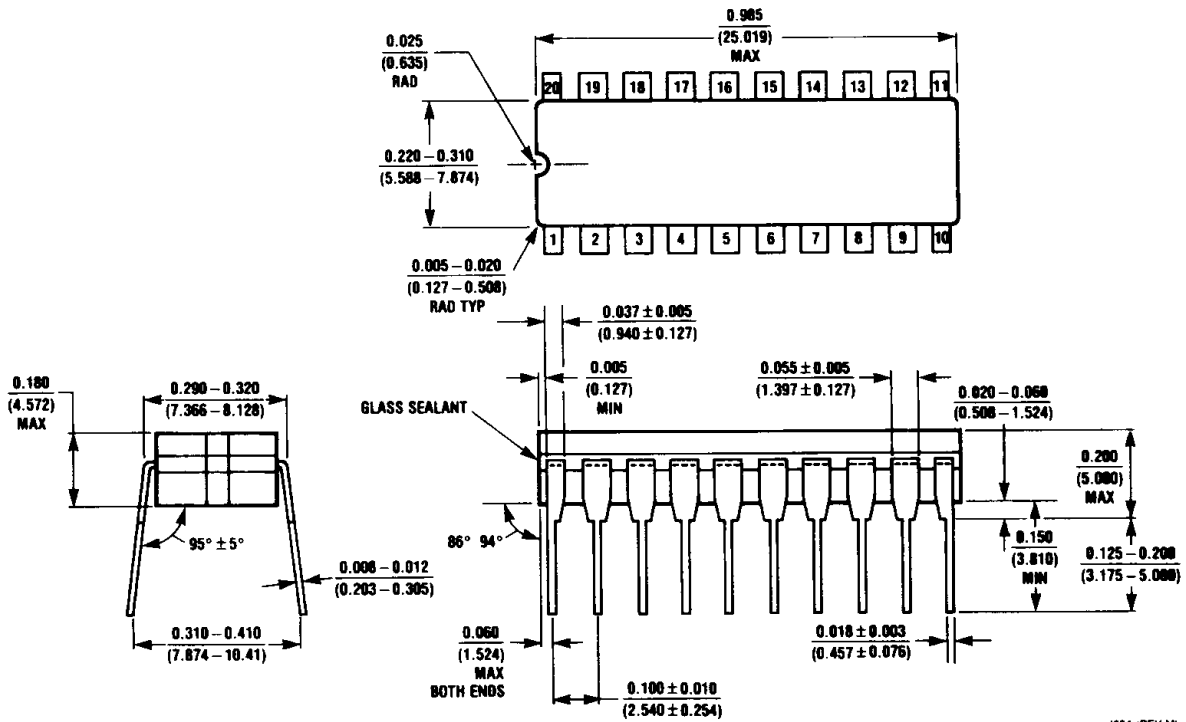
Order Number ADC08238BIJ, ADC08238CIJ or ADC08238CMJ NS Package Number J20A
