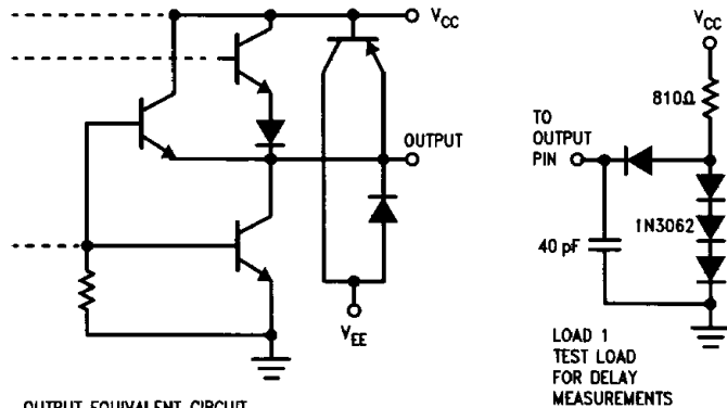
FIGURE 4. Simplified Digital Output Circuit
