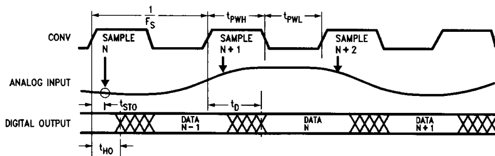
FIGURE 1. Timing Diagram
