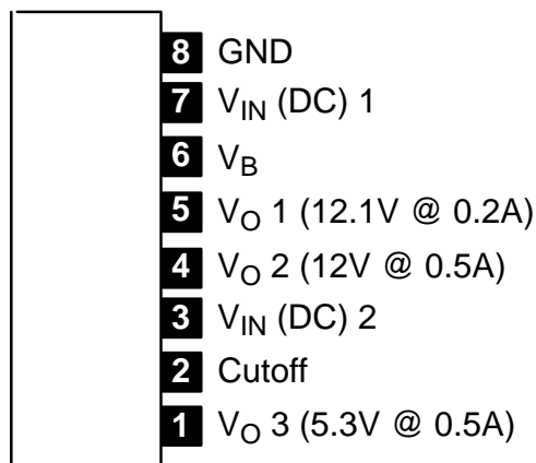
Pin Connection Diagram (Front View)
