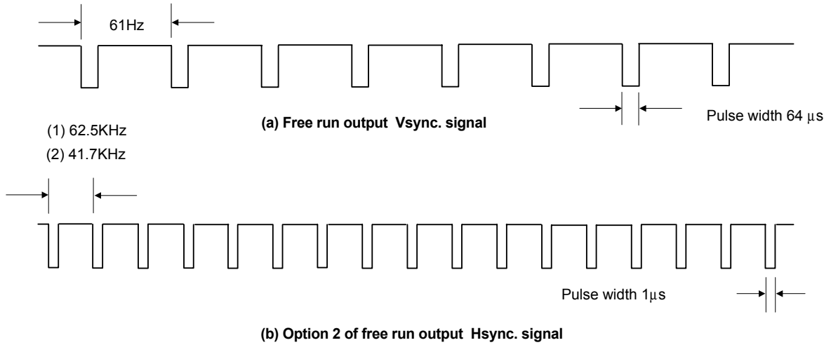
Figure 20. Free Running Sync. Waveform
