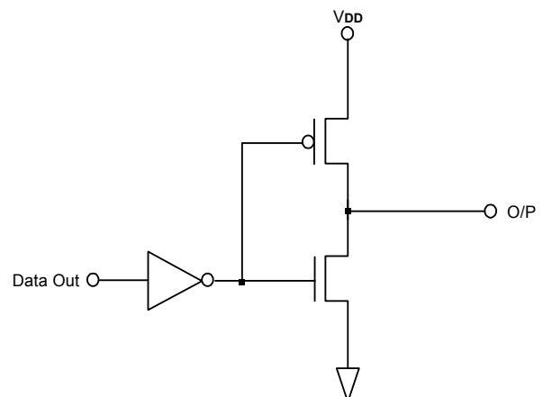
Figure 8. Output Structure
