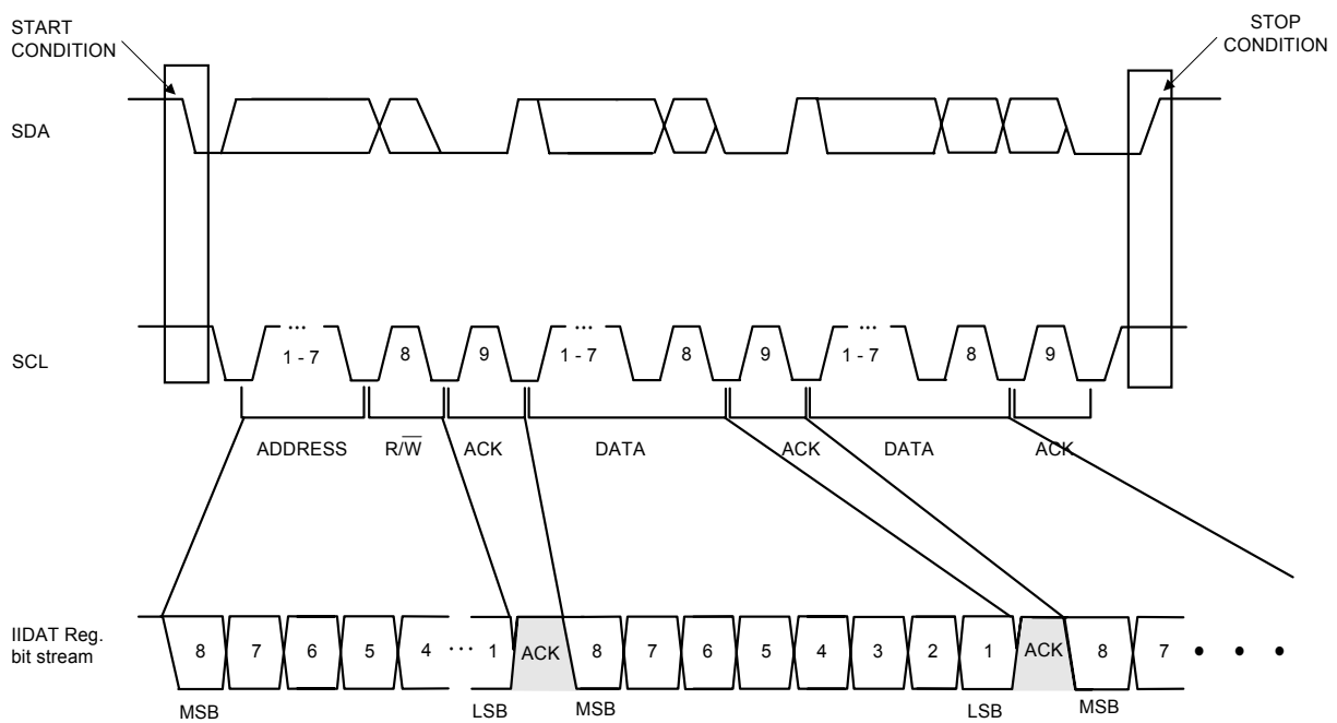
Figure 23. DDC2B Data Transfer
