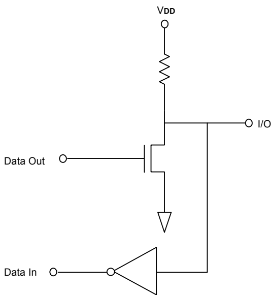
Figure 6. I/O Structure
