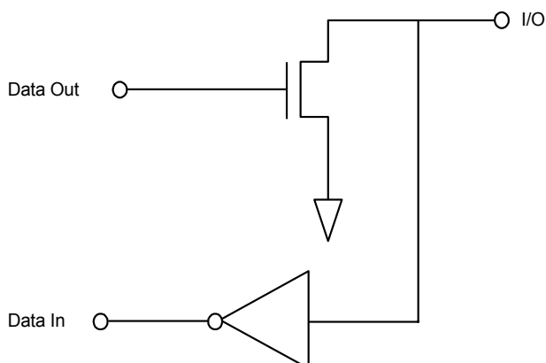
Figure 11. Open Drain I/O Structure
