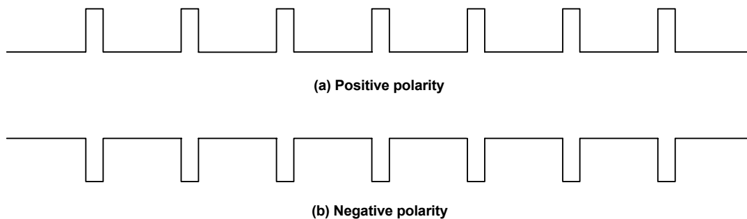
Figure 12. Separate H Sync. Waveform
