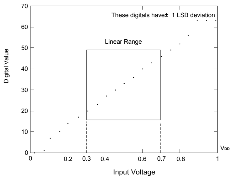
Figure 3. A/D Converter Linearity Diagram
