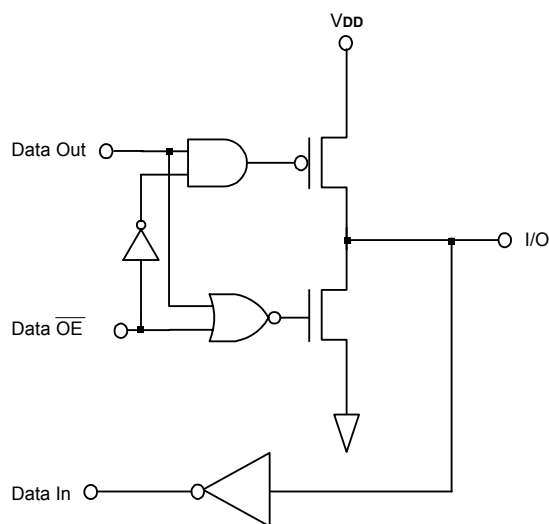
Figure 10. I/O Structure
