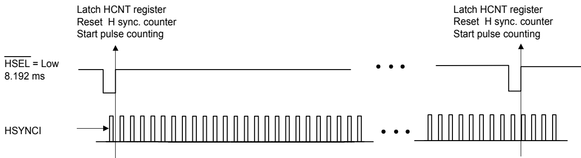
Figure 16. Hsync Counter Operation Using 8.192ms Time Interval
