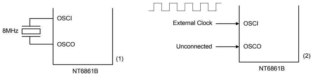
Figure 2. Oscillator Connections
