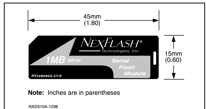
Figure 1. Serial Flash Module
