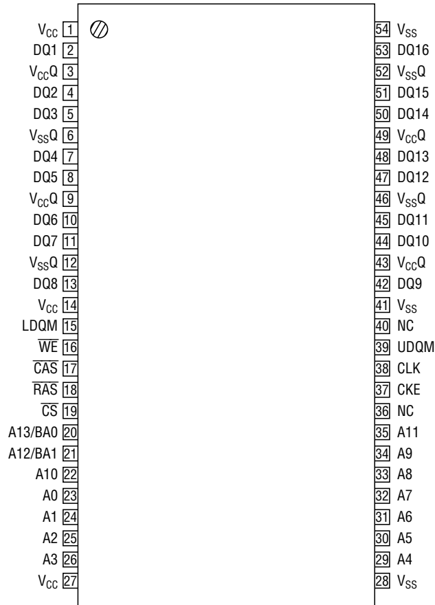
54-Pin Plastic TSOP (II) (K Type)
