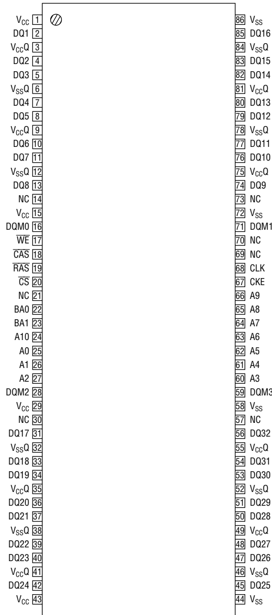
86-Pin Plastic TSOP (II) (K Type)
