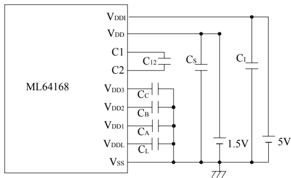
ML64168 1.5V Version.(The LCD bias is regulated.)
