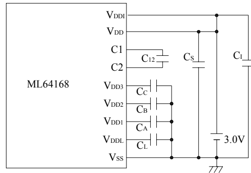
ML64168 3.0V Version.(The LCD bias is regulated.)
