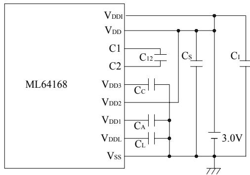
ML64168 3.0V Version
