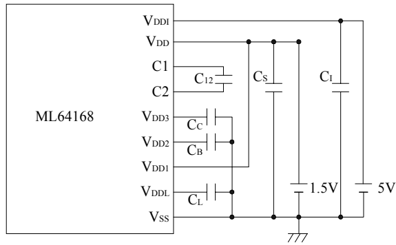
ML64168 1.5V Version
