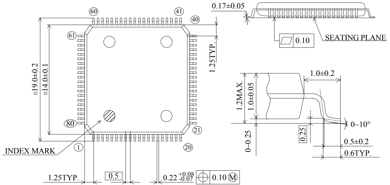
Figure C-3 80-Pin QFP:TB Package Dimension Diagram
