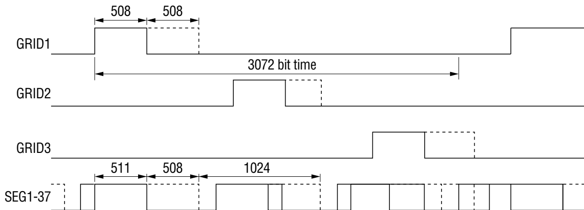
Figure 6. Duty Cycle Timing (1/3 Duty Mode)
