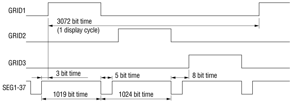
Figure 5. Duty Cycle Timing (1/3 Duty Mode)
