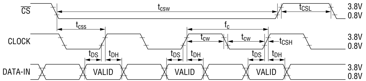
Figure 1. Data Input Timing
