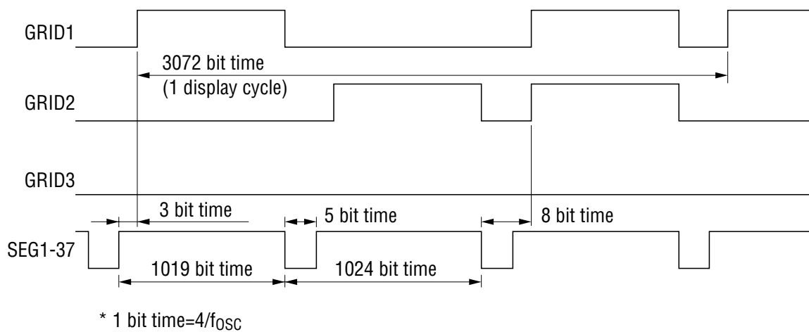
Figure 4. Duty Cycle Timing (Universal VFD Mode)
