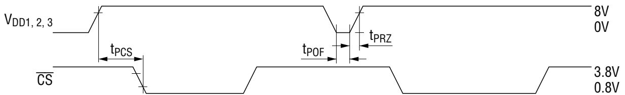
Figure 3. Power-on Timing
