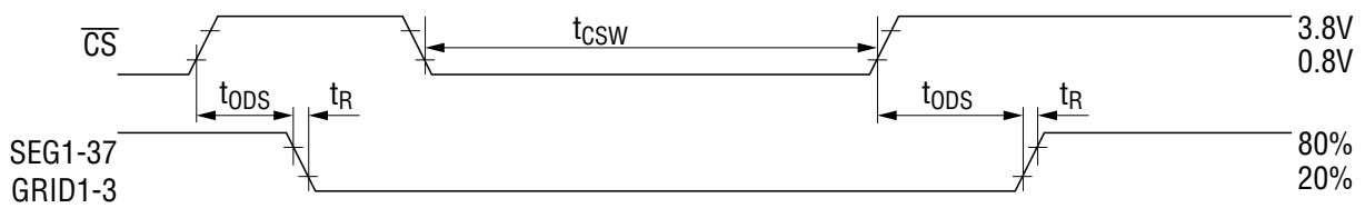
Figure 2. SEG or GRID Driver Output Timing
