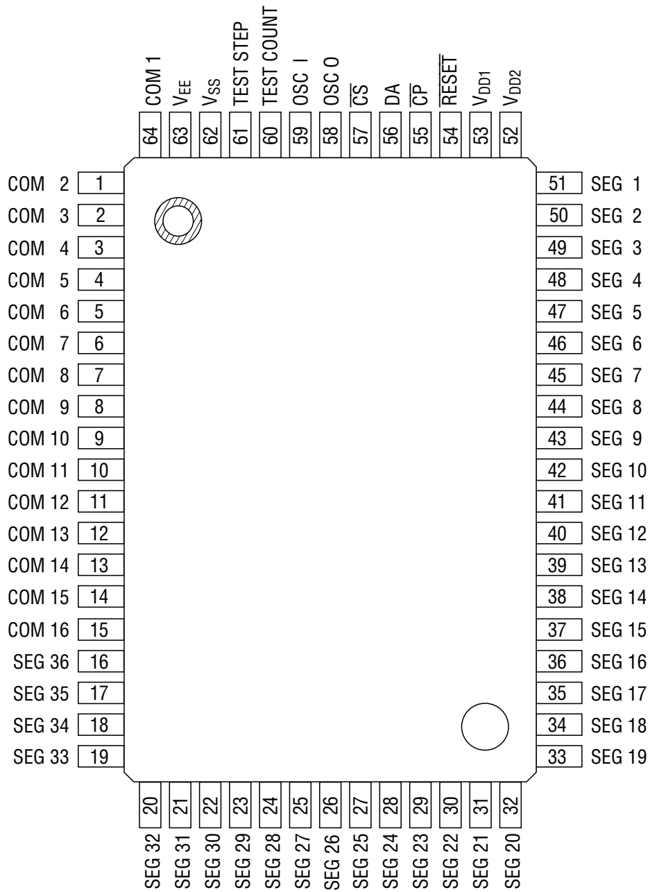
64-Pin Plastic QFP
