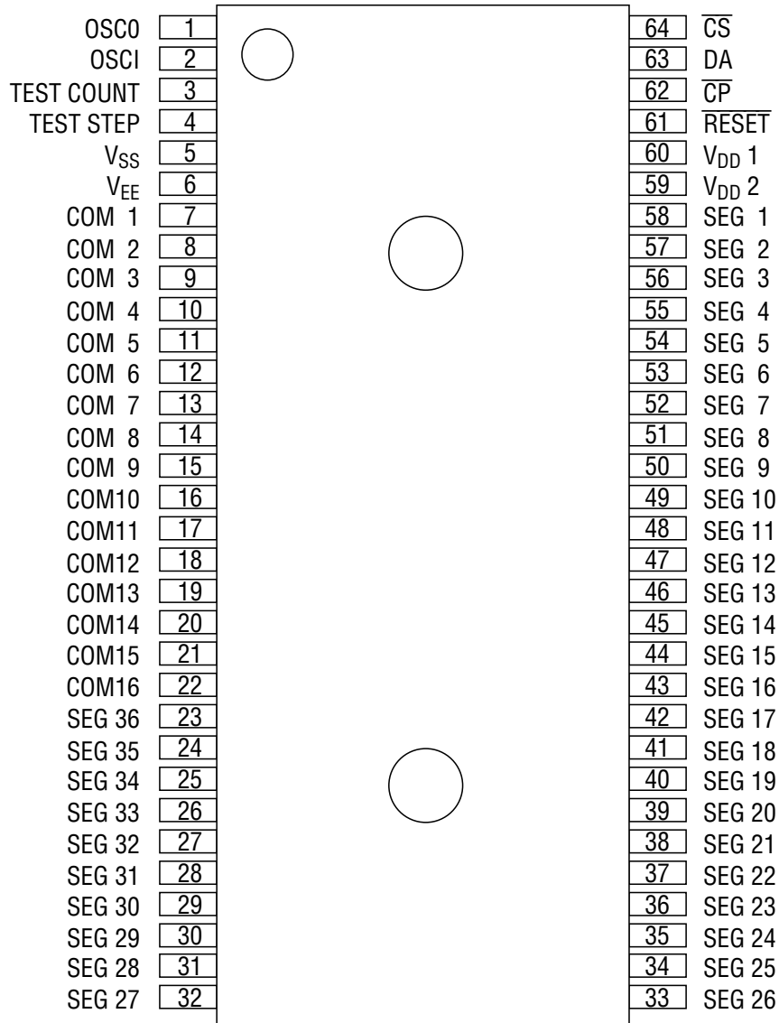
64-Pin Plastic Shrink DIP
