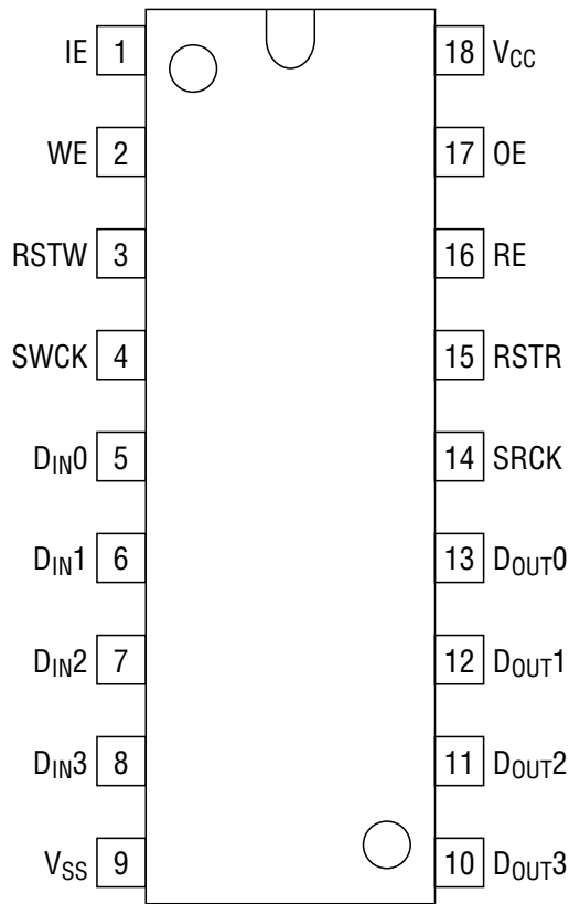
18-Pin Plastic DIP
