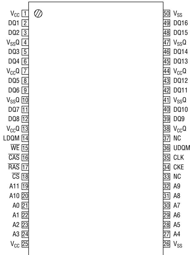
50-Pin Plastic TSOP (II) (K Type)
