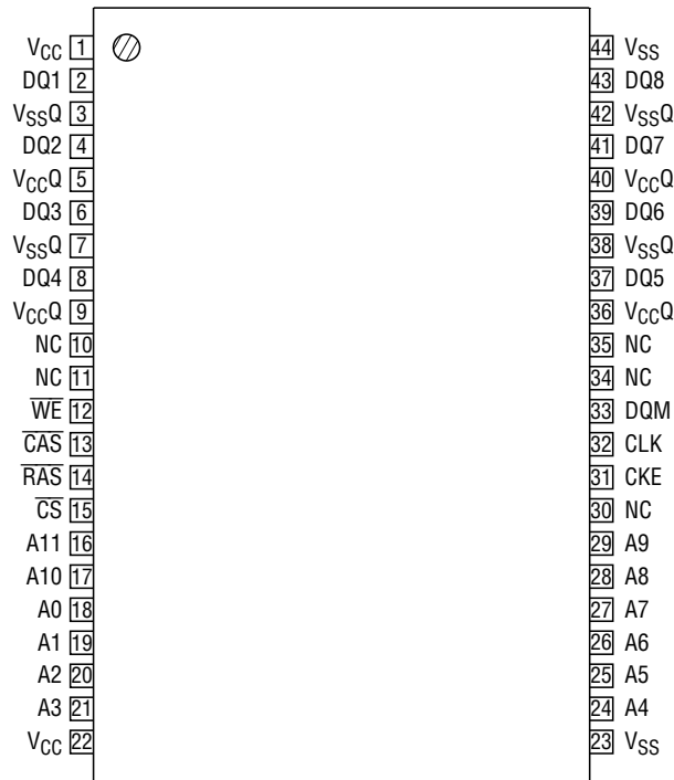
44-Pin Plastic TSOP (II) (K Type)
