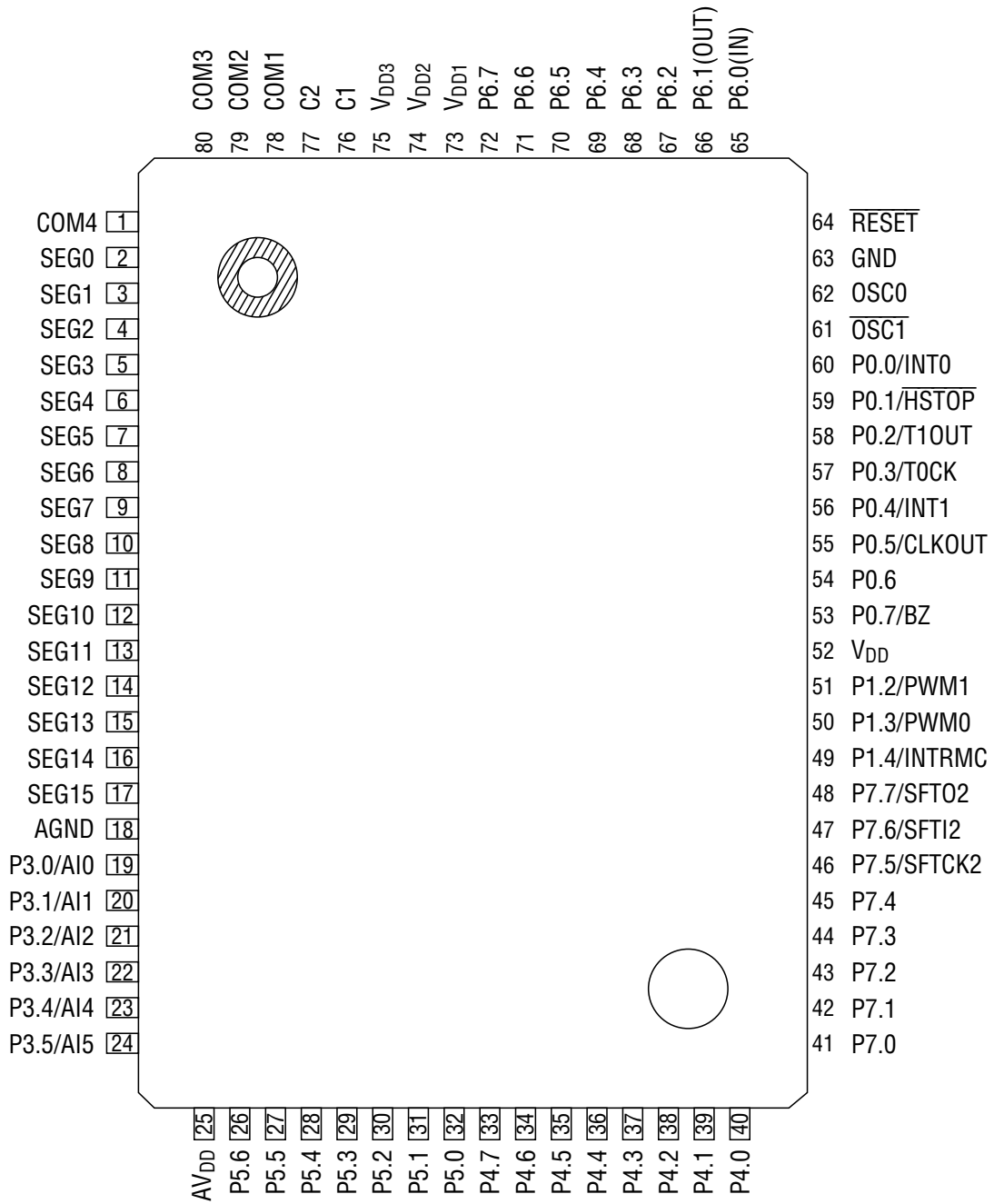
80-Pin Plastic QFP
