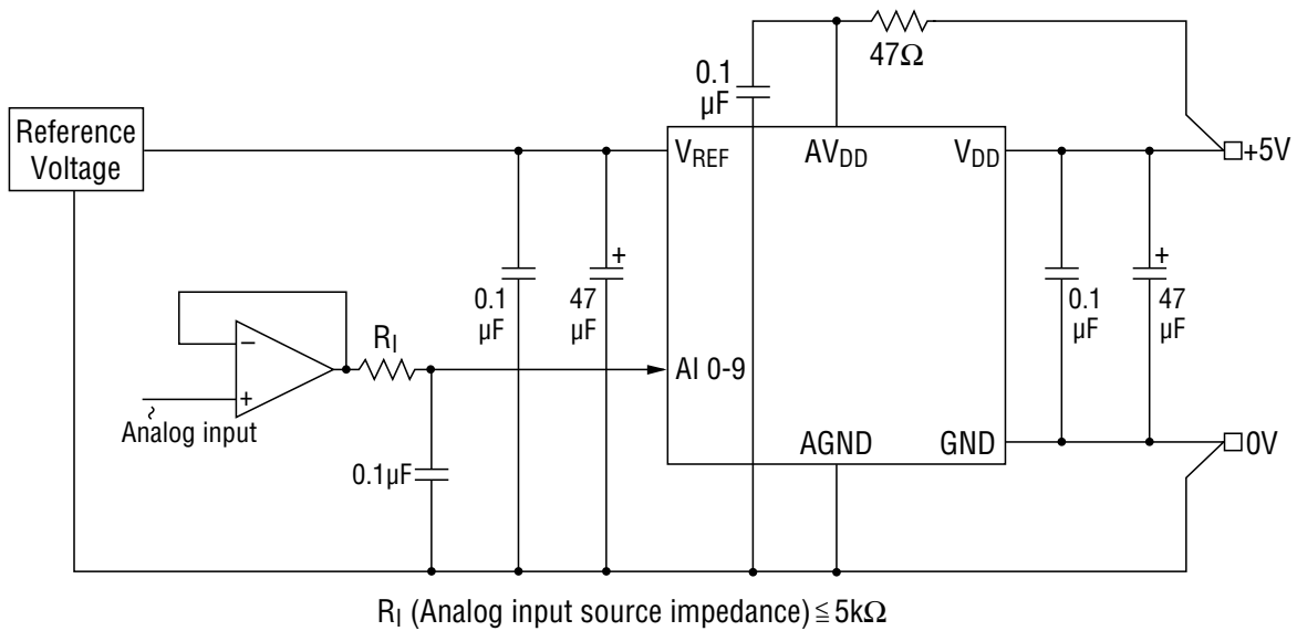
Figure 1 Recommended Circuit
