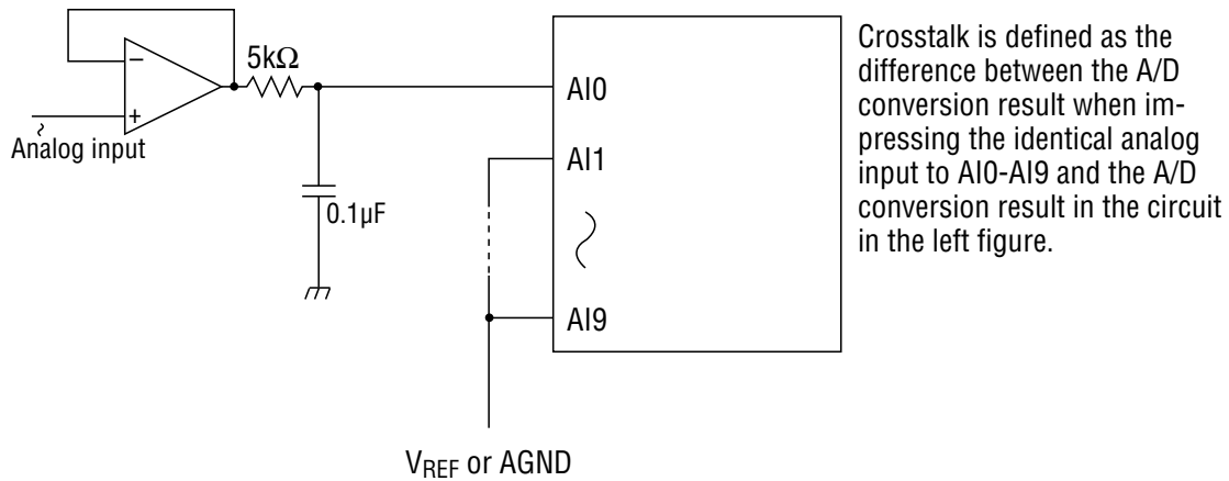
Figure 2 Crosstalk Measuring Circuit
