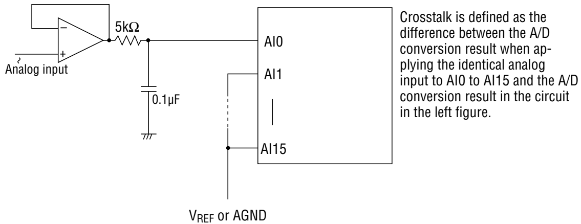
Figure 2 Crosstalk Measuring Circuit
