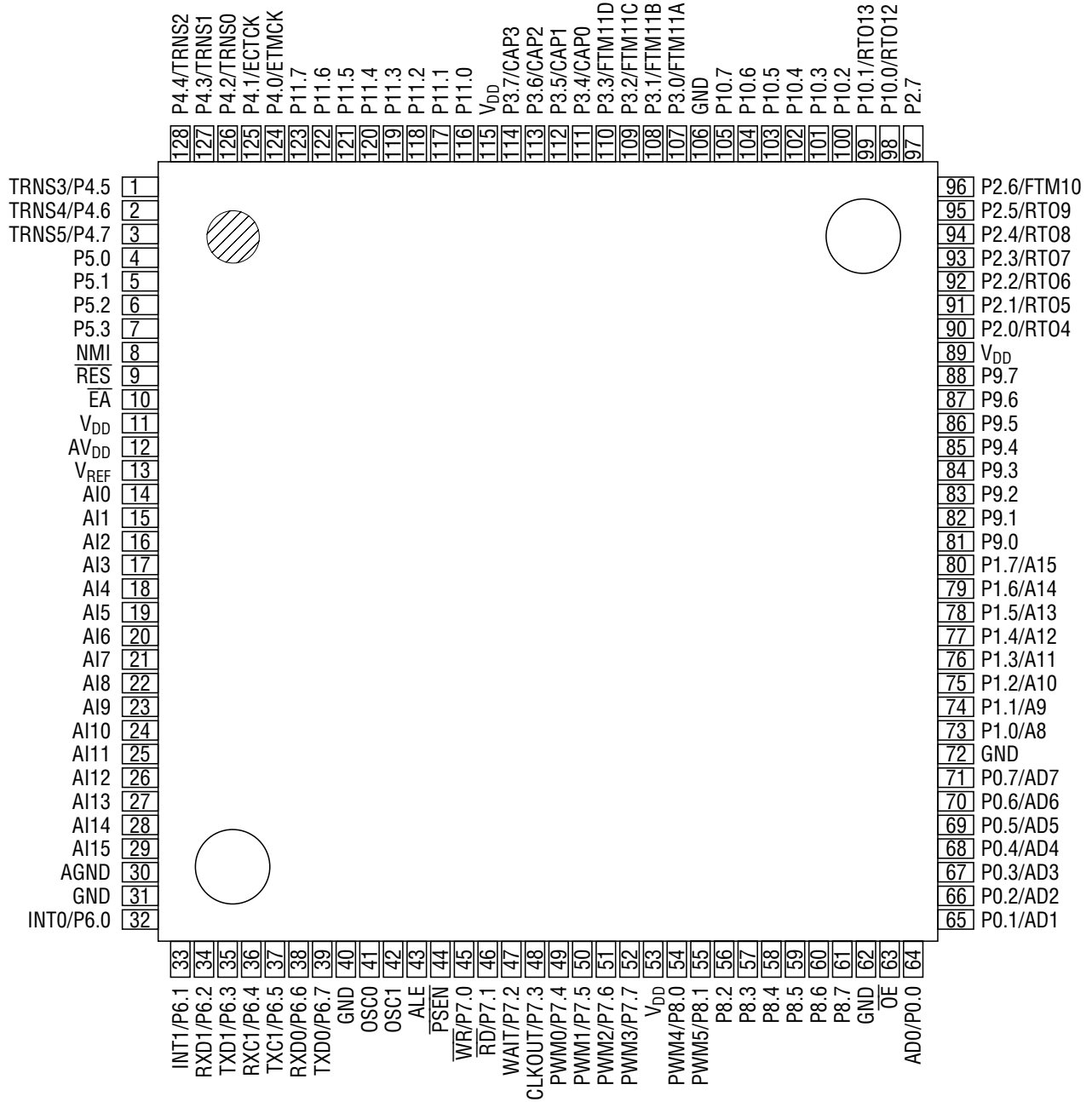
128-Pin Plastic QFP
