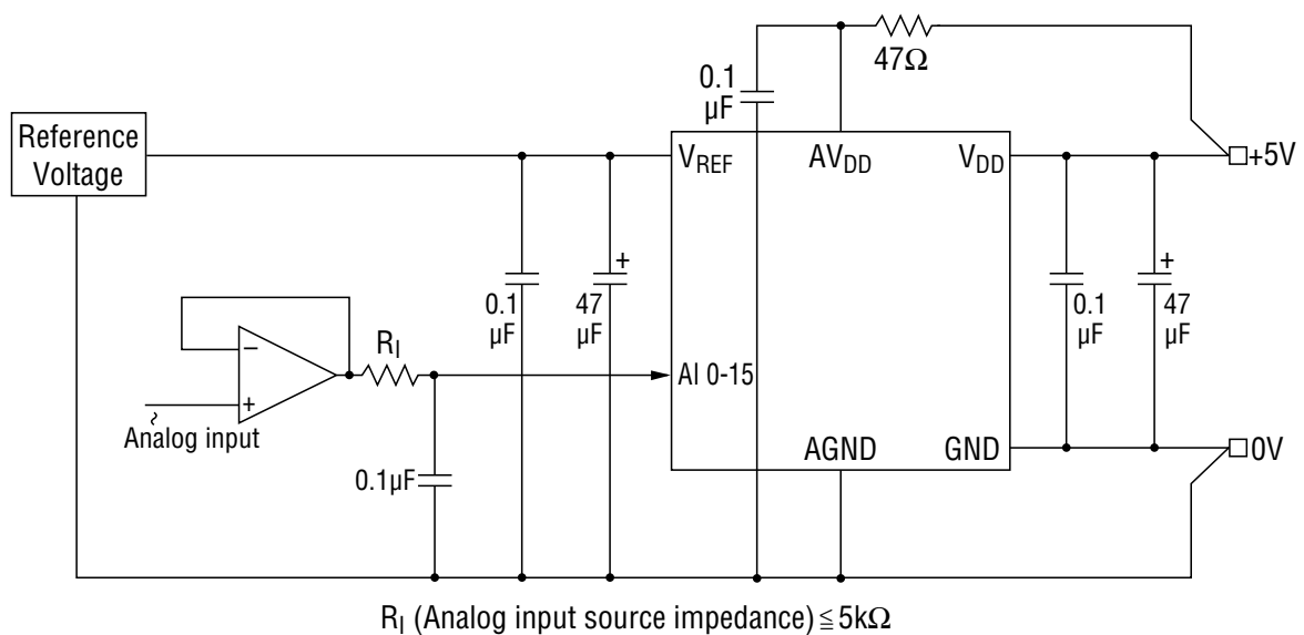
Figure 1 Recommended Circuit
