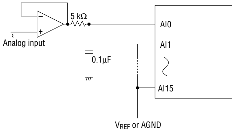
Crosstalk Measuring Circuit
