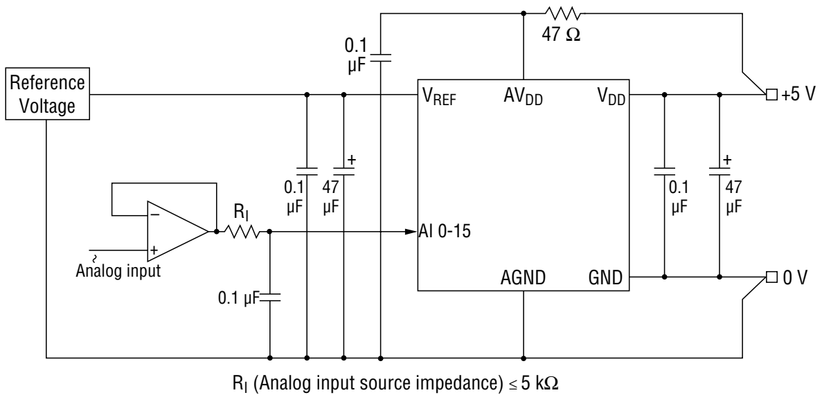
Recommended Circuit
