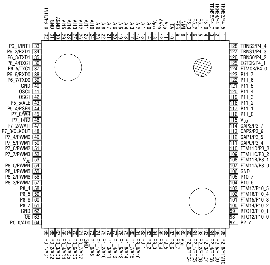
128-Pin Plastic QFP (FLAT)
