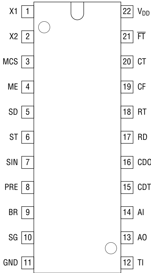
22-Pin Plastic DIP
