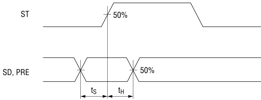
Figure 1 Input Data Timing
