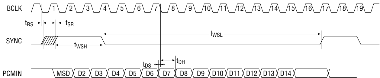
Figure 1 Basic Timing Diagram
