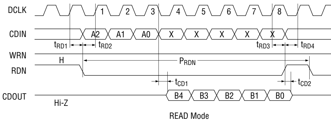
Figure 2 Processor Timing Diagram
