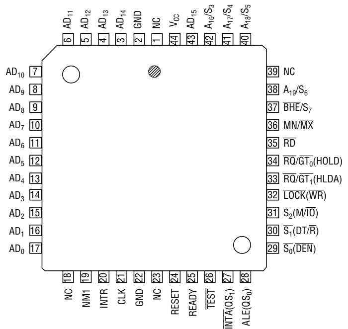
44 pin Plastic QFJ
