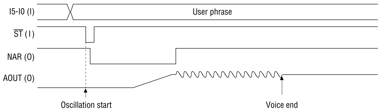
Figure 2.1 Voice Start Timing
