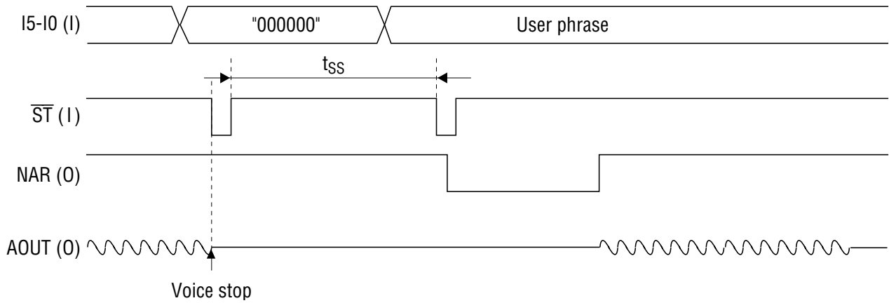
Figure 3.1 Stop Code Input Timing
