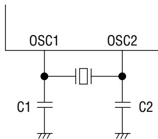
Figure 6.1 Ceramic Oscillation Diagram
