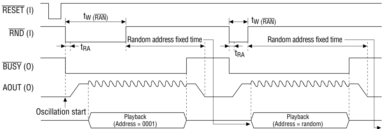
Figure 3.3 Random Address Capture
