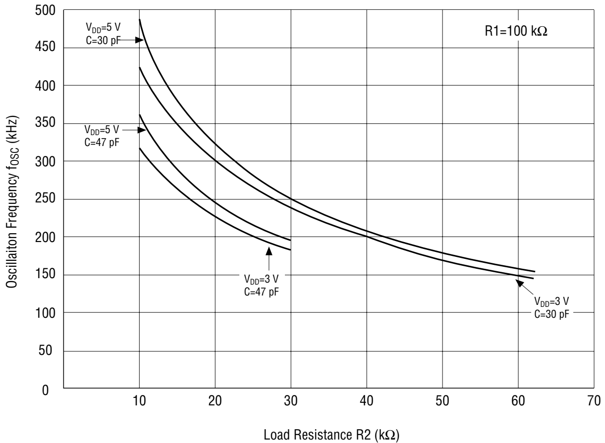
Figure 5.2 RC Oscillation Frequency Characteristics
