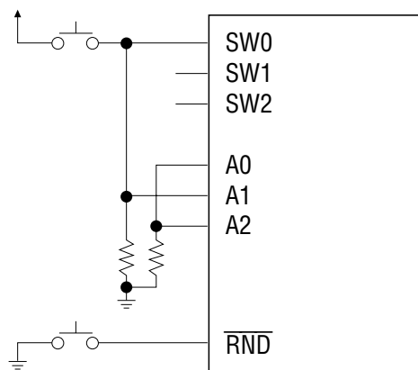
Figure 3.5 Circuit Example for Random Playback Stop
