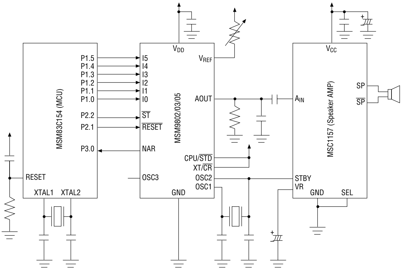
Application Circuit in Microcontroller Interface
