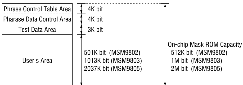
Figure 2.1 Memory Allocation of On-chip Mask ROM
