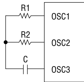
Figure 5.1 RC Oscillation
