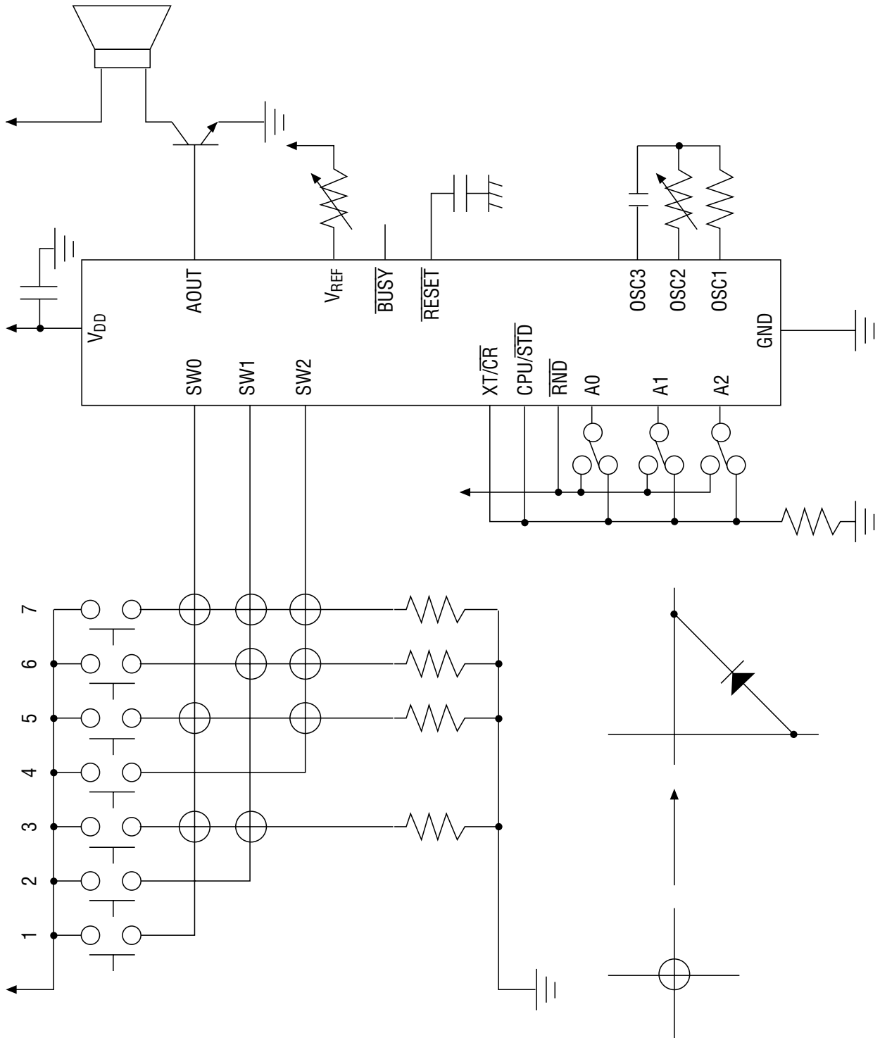
Application Circuit Using Switches
