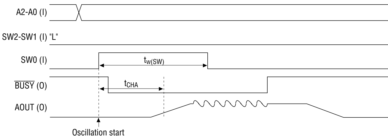
Figure 3.1 SW Input Interface Single-Phrase Playback Timing
