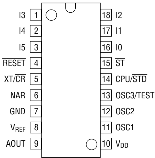
18-Pin Plastic DIP
