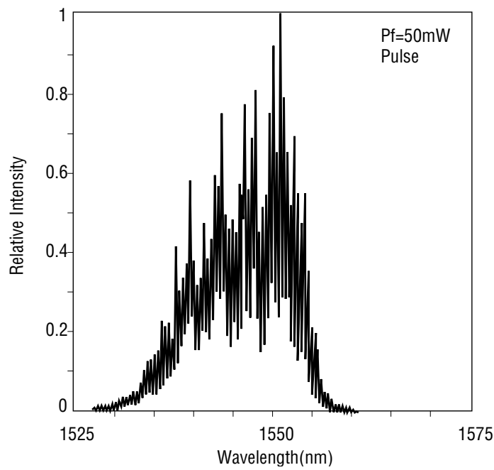
Oscillation Spectrum
