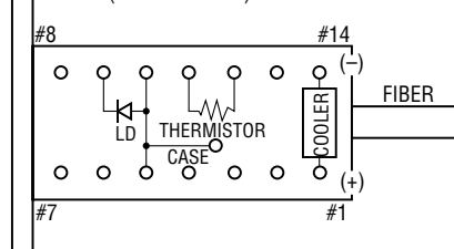
TERMINAL CONNECTION (BOTTOM VIEW)
