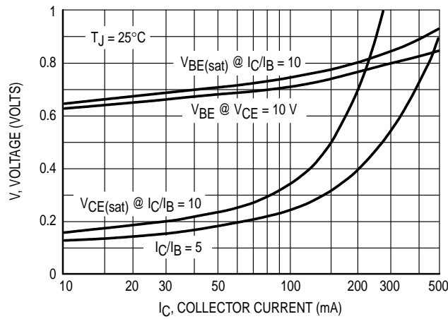
Figure 2. "On" Voltages
