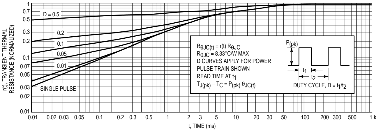
Figure 5. Thermal Response
