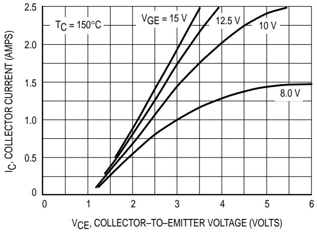
Figure 2. Saturation Characteristics
