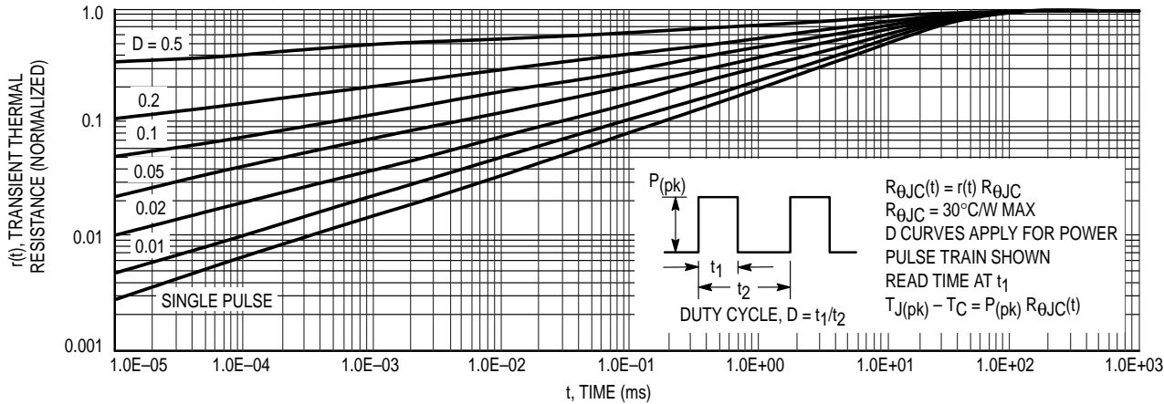
Figure 12. Typical Thermal Response
