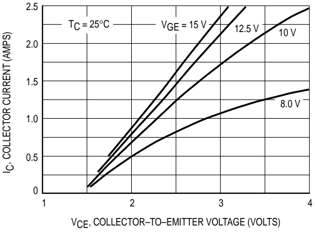
Figure 1. Saturation Characteristics
