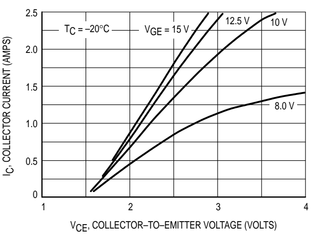
Figure 3. Saturation Characteristics
