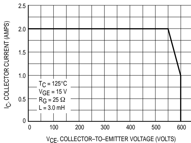
Figure 11. Minimum Turn-Off Safe Operating Area
