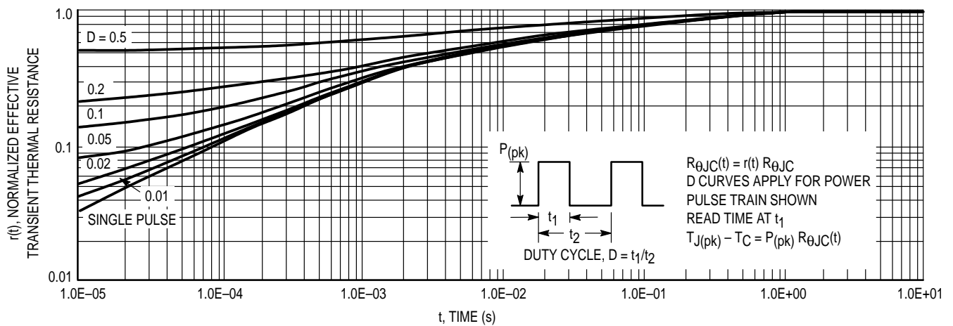
Figure 10. Thermal Response
