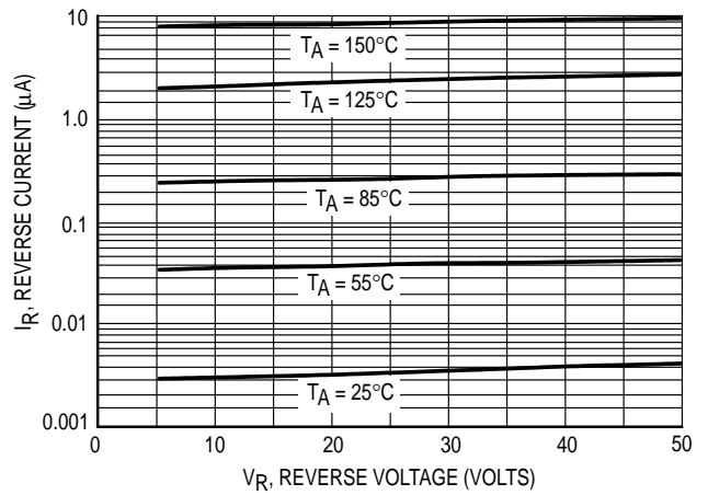
Figure 2. Reverse Current
