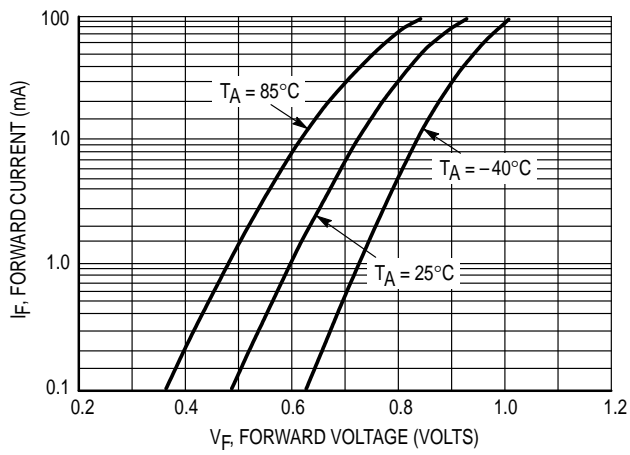
Figure 1. Forward Voltage
