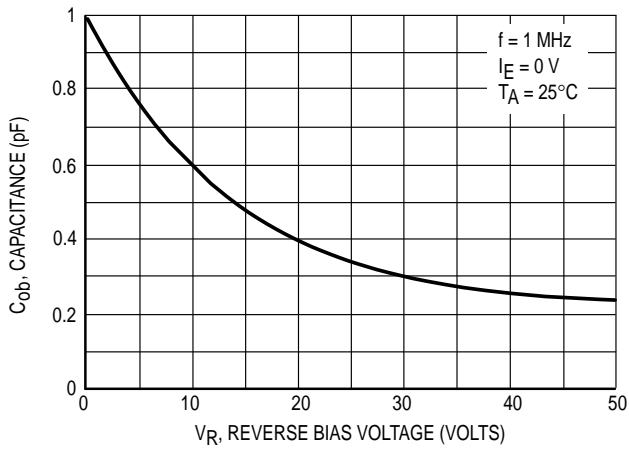
Figure 24. Output Capacitance
