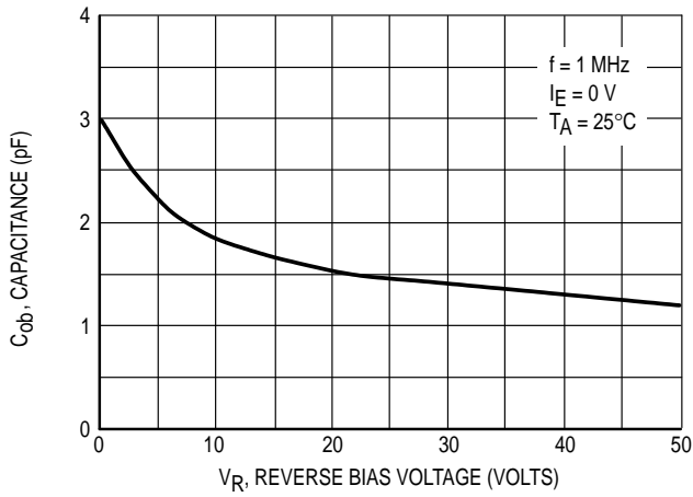
Figure 14. Output Capacitance
