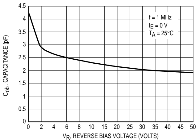
Figure 39. Output Capacitance
