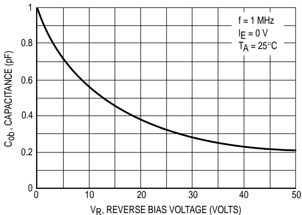
Figure 29. Output Capacitance
