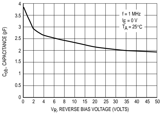
Figure 34. Output Capacitance
