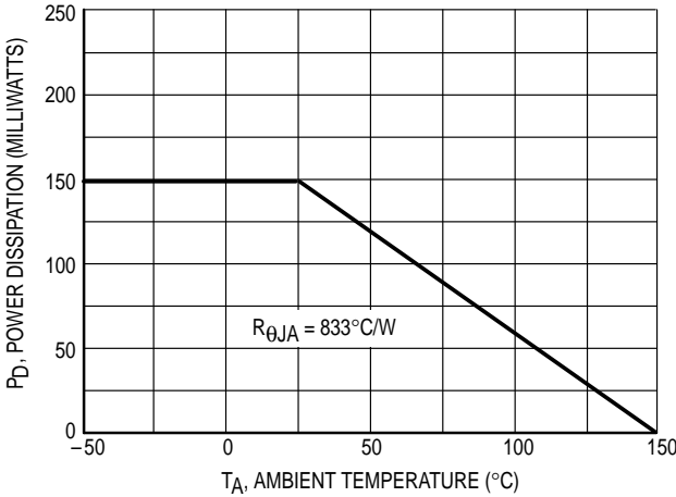
Figure 1. Derating Curve
