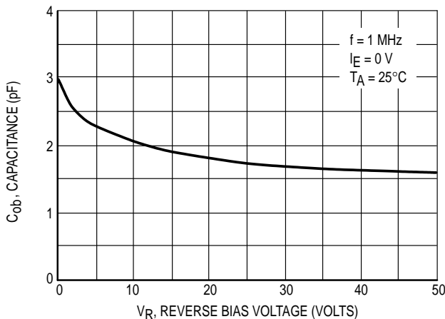
Figure 9. Output Capacitance
