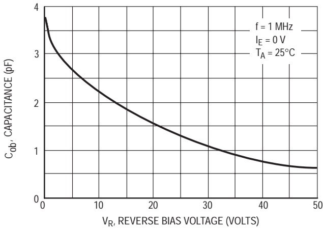
Figure 5. Output Capacitance
