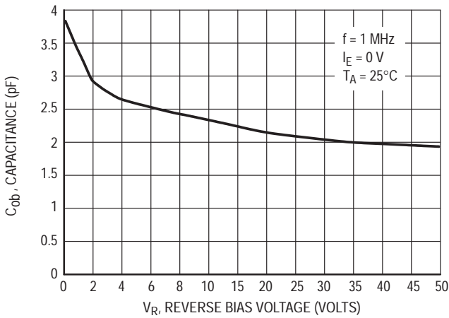
Figure 20. Output Capacitance
