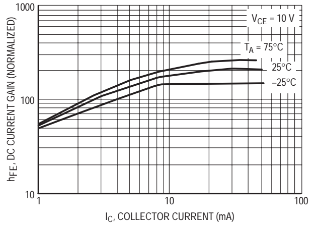
Figure 14. DC Current Gain
