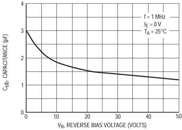
Figure 10. Output Capacitance
