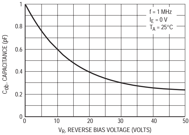
Figure 15. Output Capacitance
