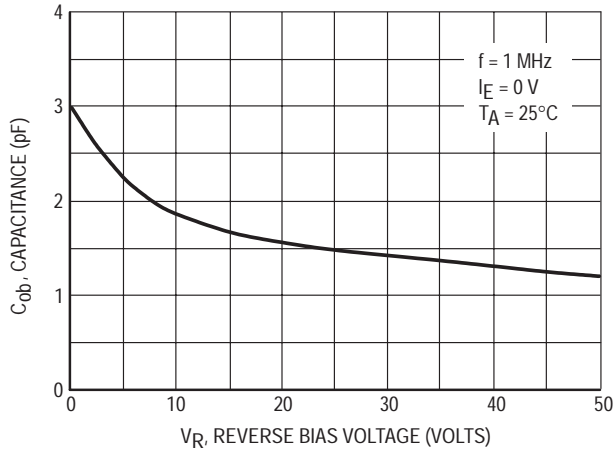
Figure 9. Output Capacitance
