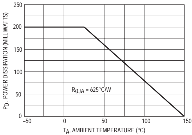
Figure 1. Derating Curve
