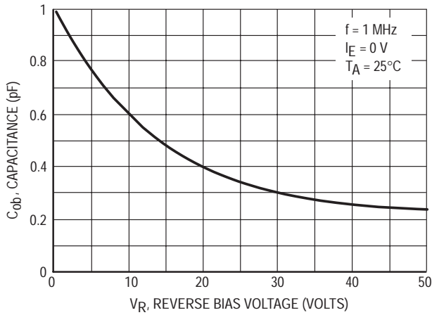
Figure 14. Output Capacitance
