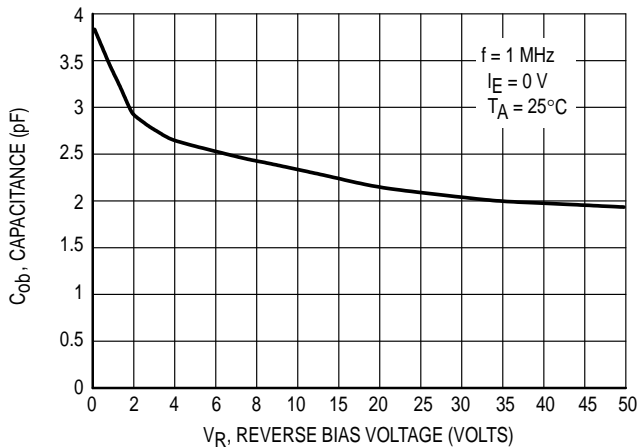
Figure 19. Output Capacitance
