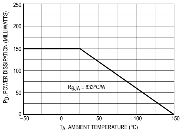
Figure 1. Derating Curve
