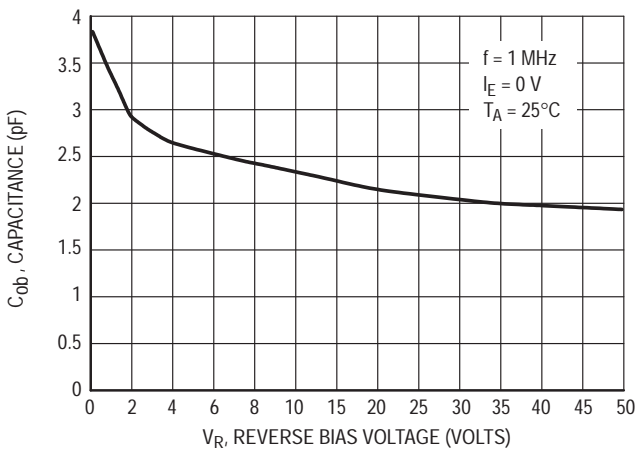
Figure 19. Output Capacitance
