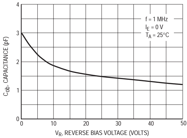
Figure 9. Output Capacitance
