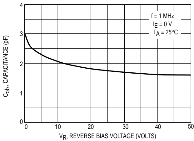
Figure 4. Output Capacitance
