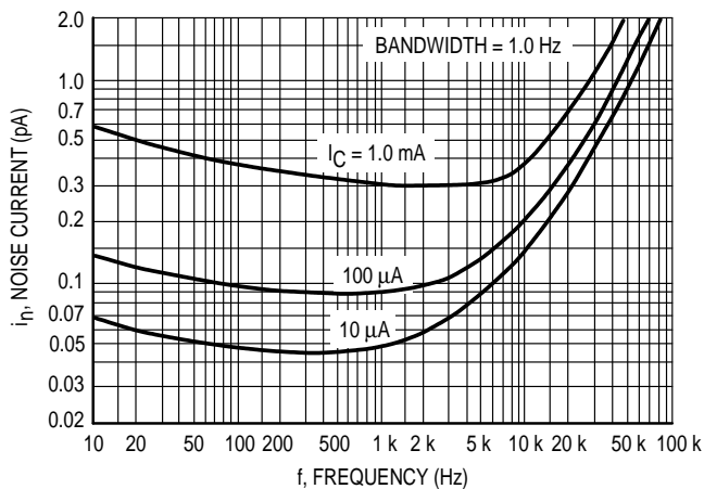
Figure 3. Noise Current
