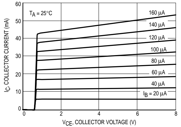
Figure 2. IC – VCE
