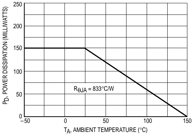
Figure 1. Derating Curve
