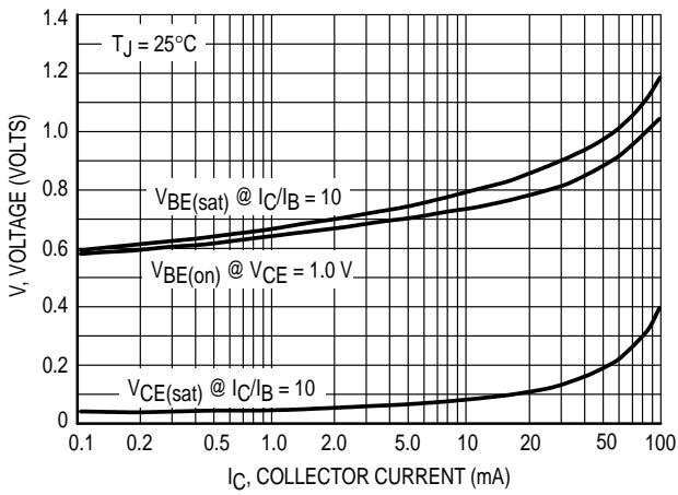
Figure 10. "On" Voltages
