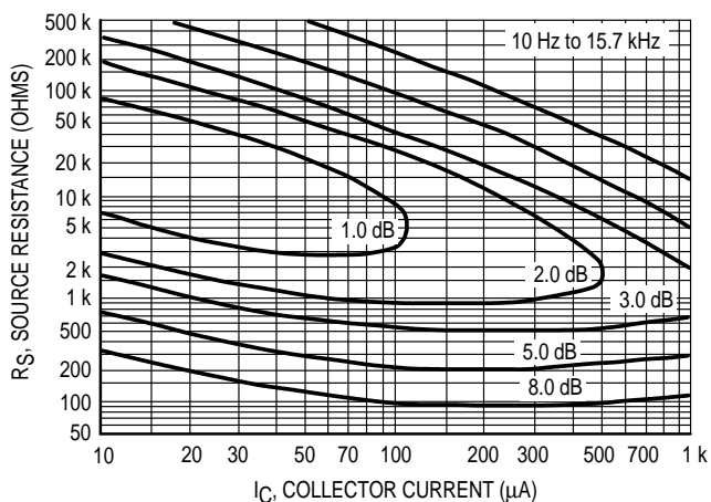
Figure 7. Wideband
