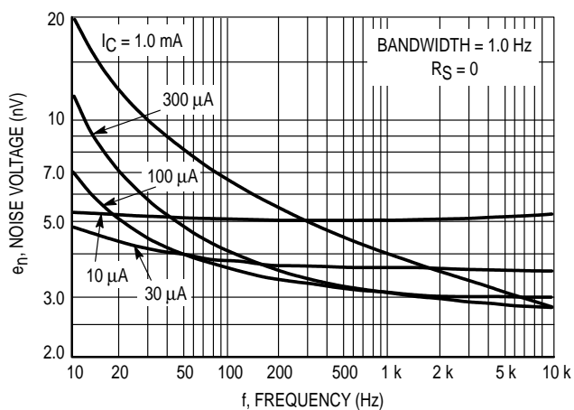
Figure 3. Noise Voltage
