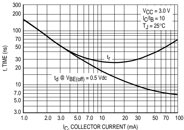
Figure 12. Turn-On Time
