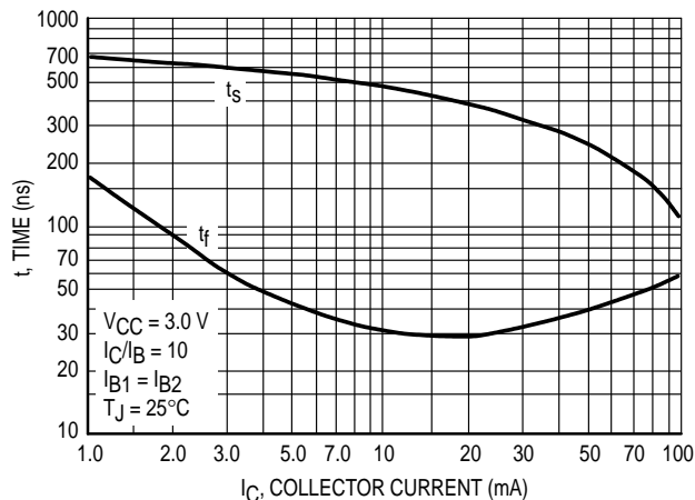
Figure 13. Turn-Off Time
