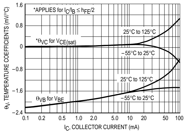
Figure 11. Temperature Coefficients
