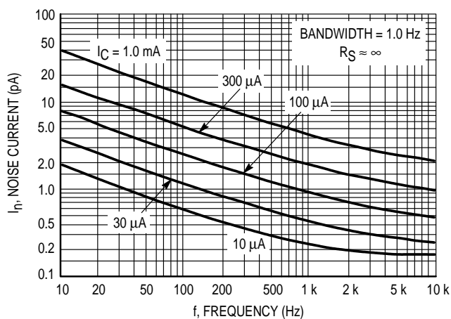
Figure 4. Noise Current
