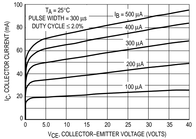
Figure 9. Collector Characteristics
