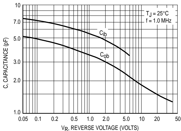
Figure 15. Capacitance
