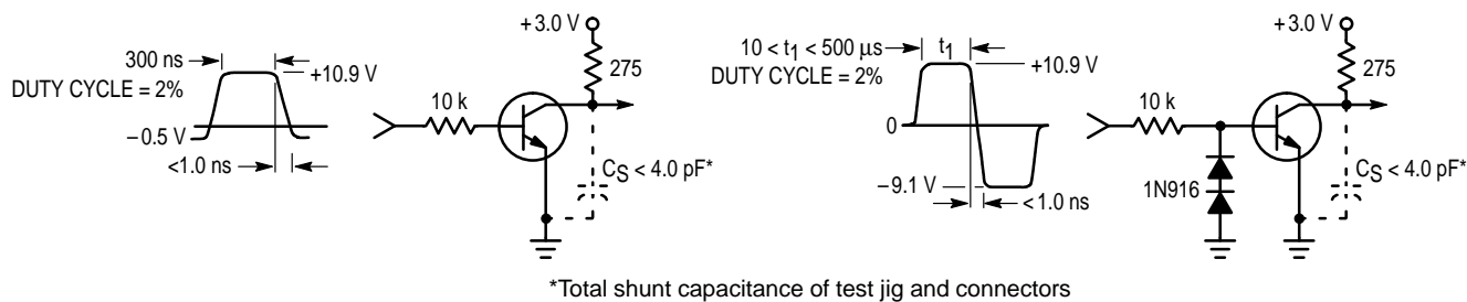
Figure 1. Turn–On Time
