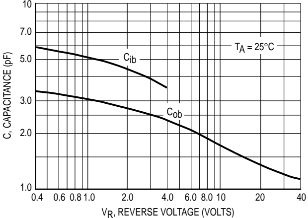
Figure 4. Capacitances
