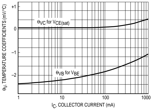
Figure 6. Temperature Coefficients
