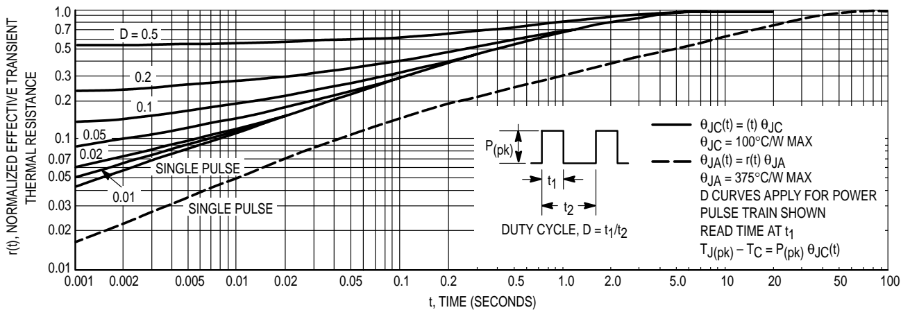
Figure 1. Thermal Response
