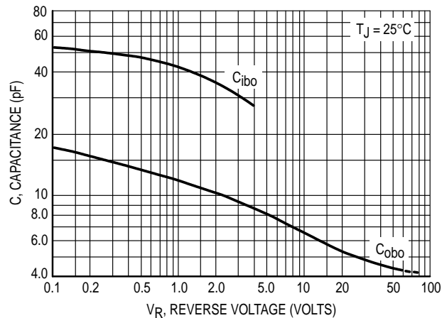
Figure 5. Capacitance
