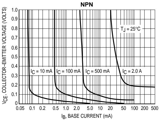
Figure 5. MPS650, MPS651 Collector Saturation Region
