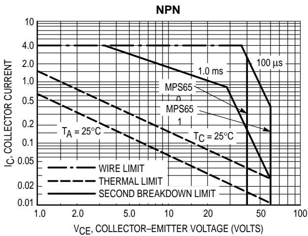
Figure 7. MPS650, MPS651 SOA, Safe Operating Area
