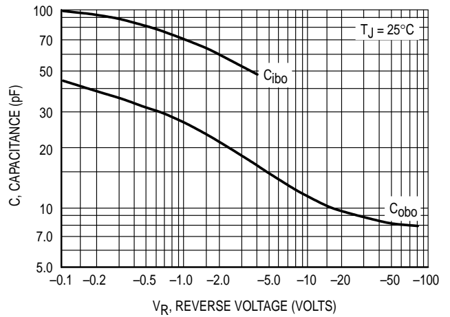
Figure 5. MPSA55/56 Capacitance
