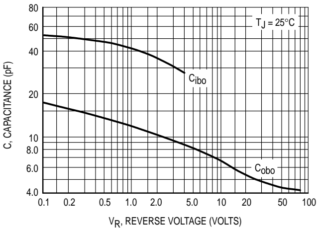
Figure 4. MPSA05/06 Capacitance
