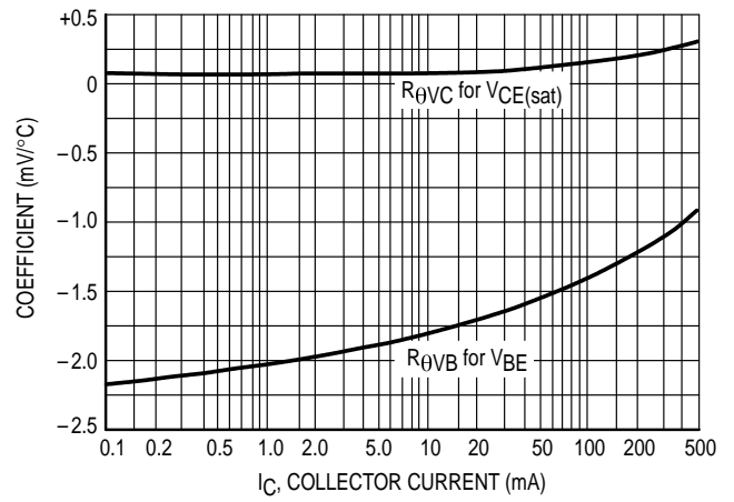
Figure 12. Temperature Coefficients
