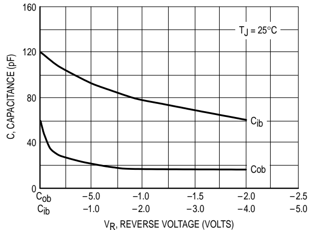
Figure 4. Capacitances
