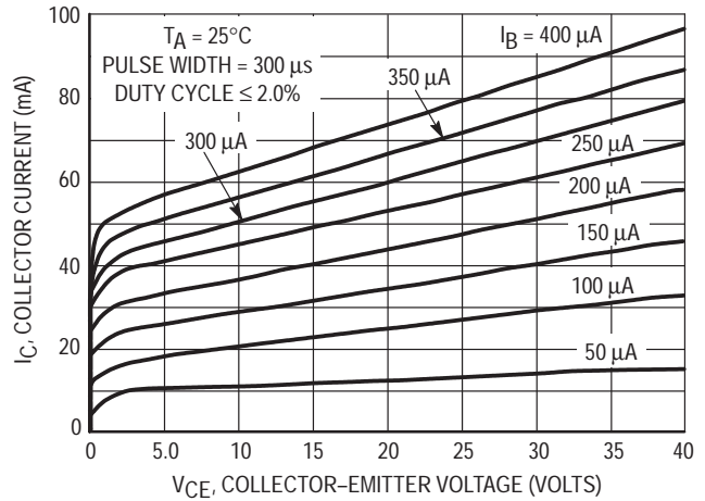
Figure 7. Collector Characteristics
