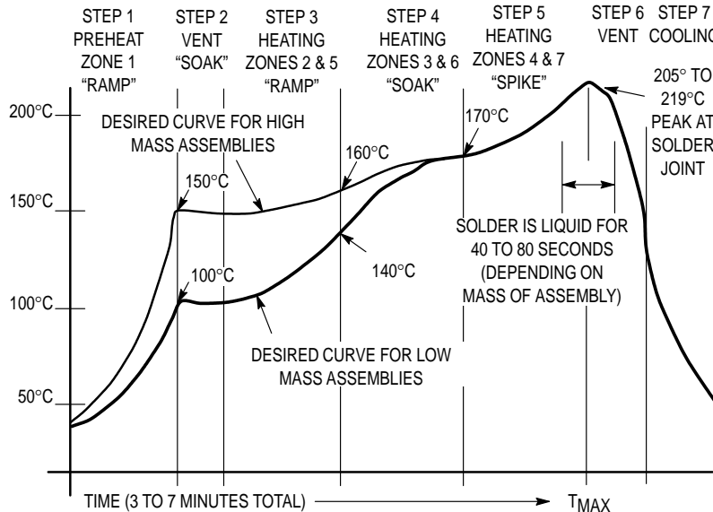
Figure 1. Typical Solder Heating Profile
