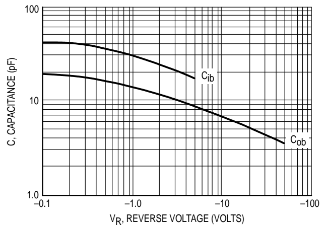
Figure 7. Capacitances
