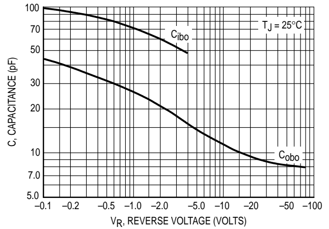
Figure 5. Capacitance
